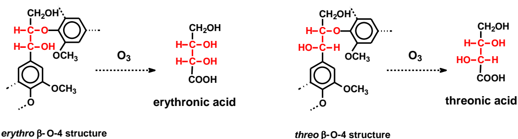
Figure 1 Formation of erythronic and threonic acids from erythro and threo β-O-4 structures by ozonation
